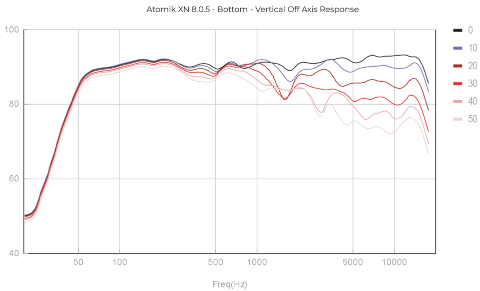
Bottom - Vertical Off Axis Response
