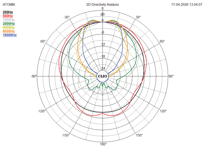
Bottom - Vertical Off Axis Response
