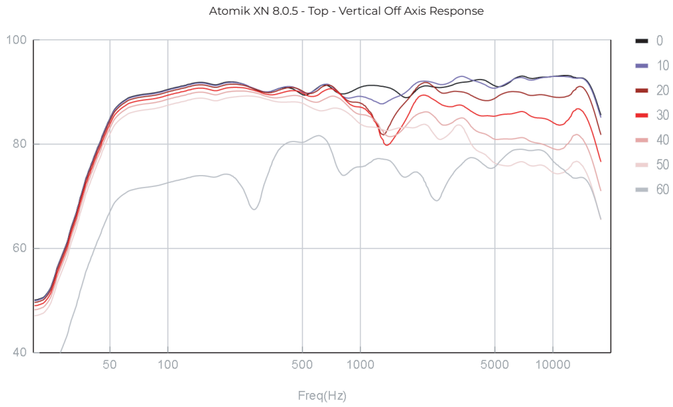
Top - Vertical Off Axis Response
