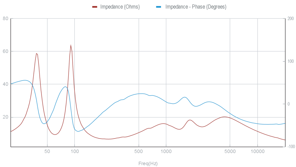
Impedance & Phase Response
